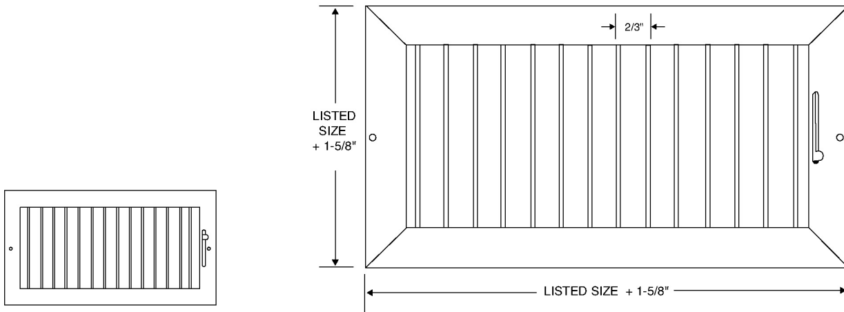
SINGLE DEFLECTION VERTICAL
